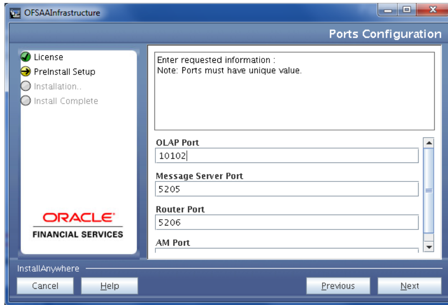
Ports Configuration_1
