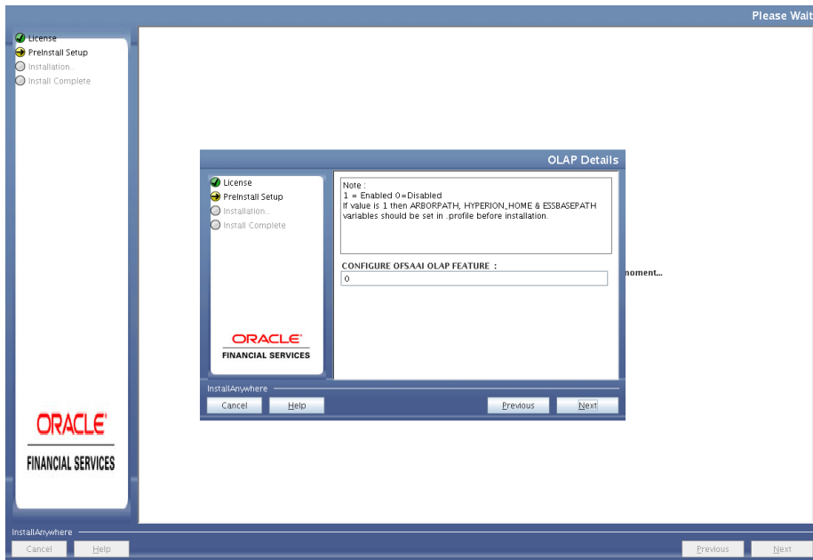
OLAP Details
