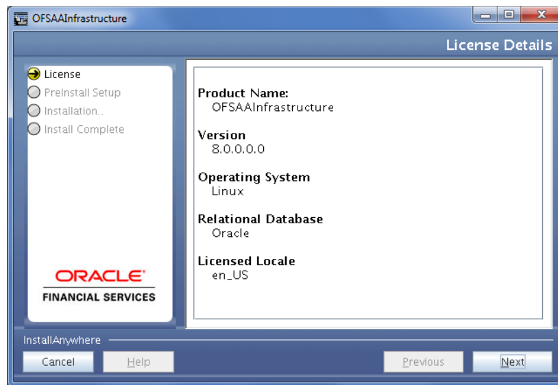
License Details
