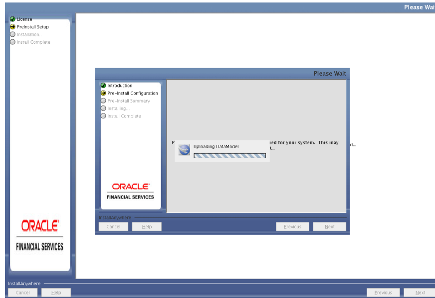
Model Upload
